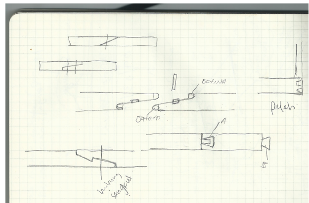
Figure 10: Sketch by modern Malay 'tukang' demonstrating a splicing joint found during disassembly and assembly, to increase the timber's length. The joint depicts the concept of male and female elements that utilise draw pins to secure the timber pieces together.
