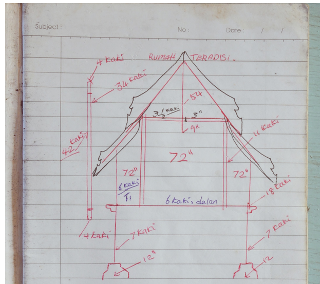
Figure 6: Sketch by the modern Malay 'tukang', outlining the dimension of each building component during the design stage in order to specify material quantity.
