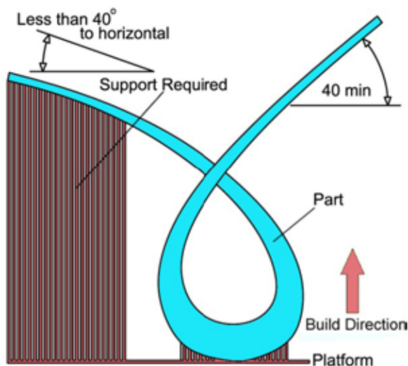
Figure 11: SLM support requirements.
